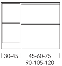
Basi lavabo a terra H.72 P.45/50
